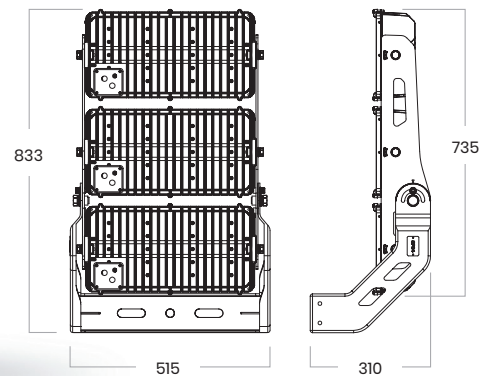
Dimensions of 1500W & 1800W
